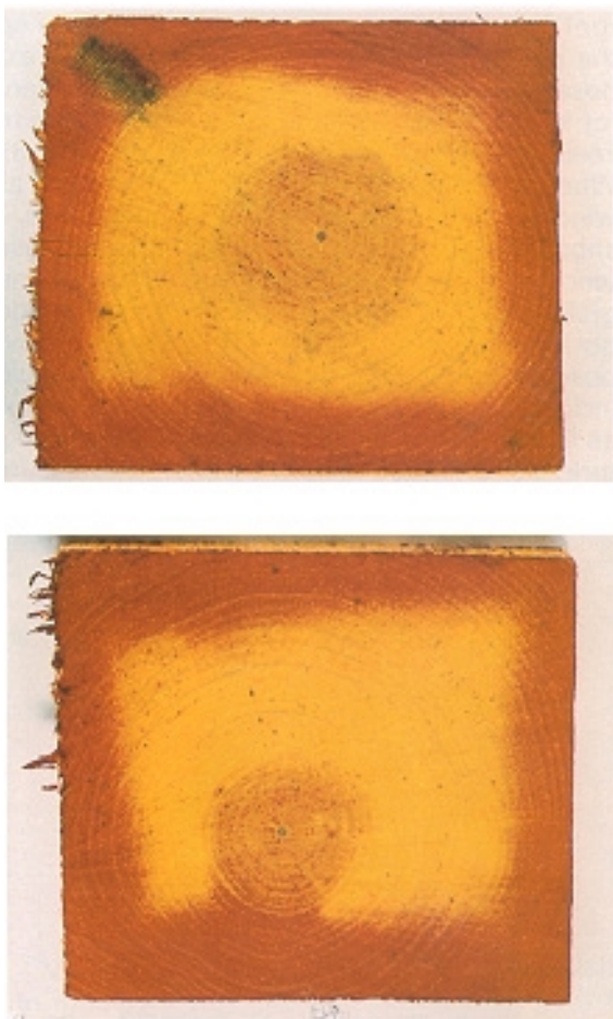
Fig. 2. Wood samples treated with Tim-Bor®, an EPA registered wood preservative. The color gradation from the surface to the center of the wood indicates the extent of treatment. (United States Borax and Chemical Corporation Photo)
